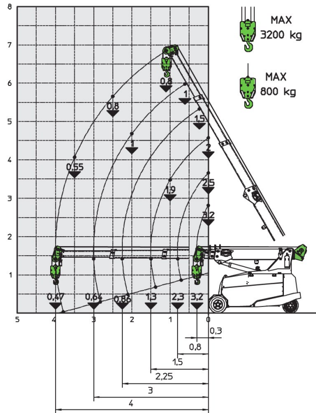
LOAD CHART HYDRAULIC WINCH
