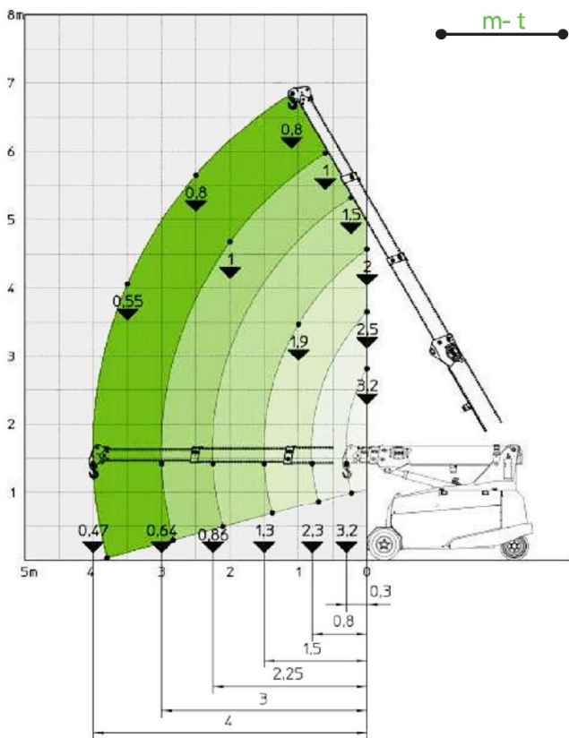
BASIC CRANE LAOD CHART
